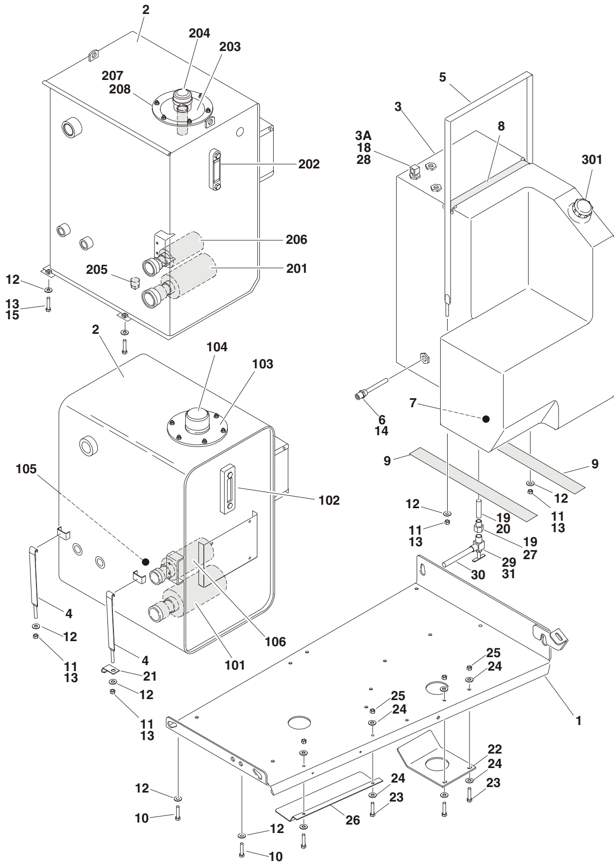
FIGURE 2-18. TANK INSTALLATIONS
