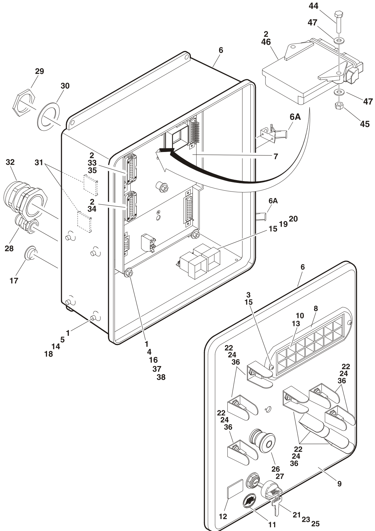
FIGURE 2-22. GROUND CONTROL BOX ASSEMBLY (WITHOUT UGM)
