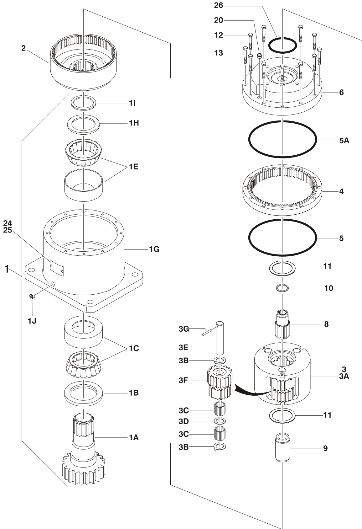
FIGURE 2-6. SWING MOTOR/HUB ASSEMBLY (SN 0300069000 TO SN 0300134353)
