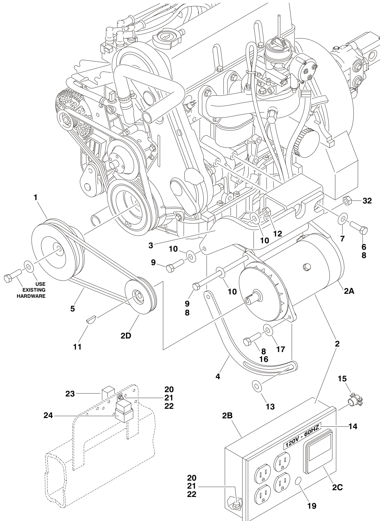
FIGURE 2-30. 2500W GENERATOR INSTALLATION - FORD MACHINES (OPTIONAL) (SN 0300069000 TO SN 0300077500)
