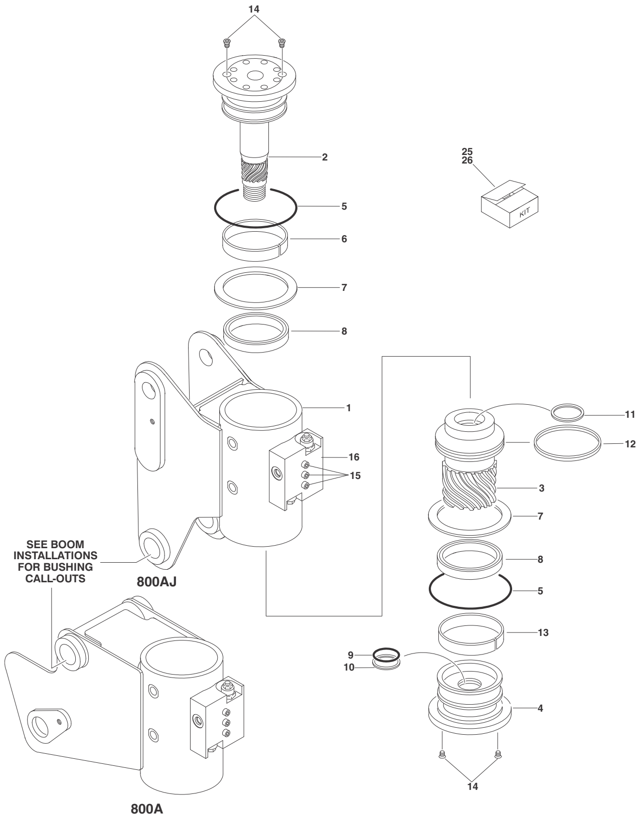
FIGURE 3-6. ROTATOR ASSEMBLY (SIDE ENTRY PLATFORM)
