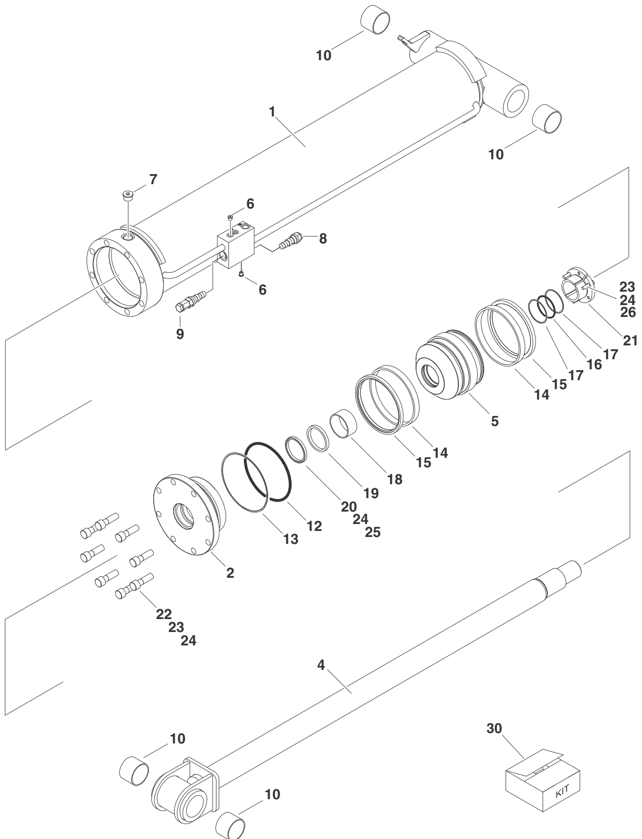
FIGURE 5-5. LIFT CYLINDER ASSEMBLY - TOWER BOOM
