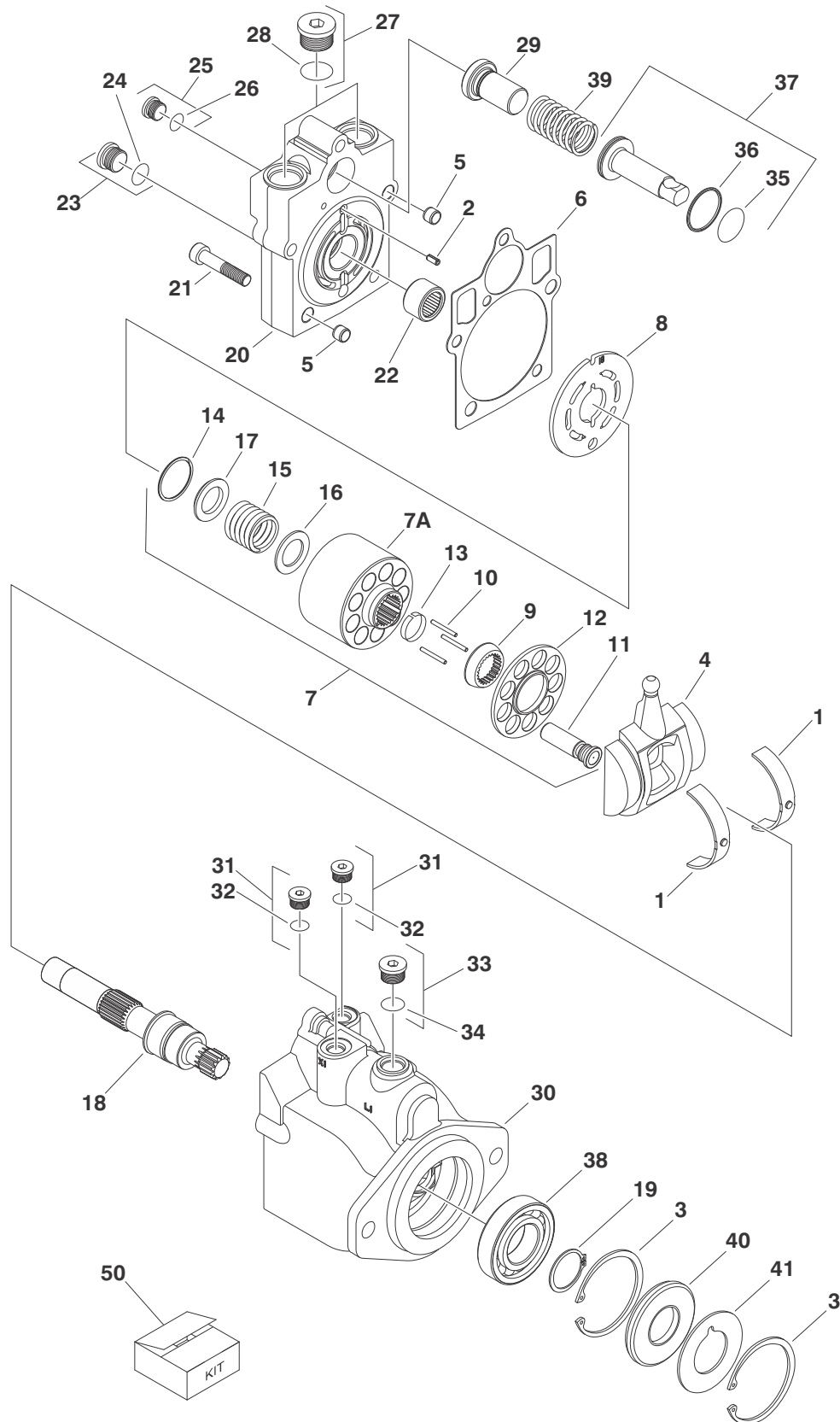
FIGURE 1-7. DRIVE MOTOR ASSEMBLY (SERVICE REPLACEMENT) (SN 0300083332 TO SN 0300140000) (5 BOLT ASSEMBLY)
