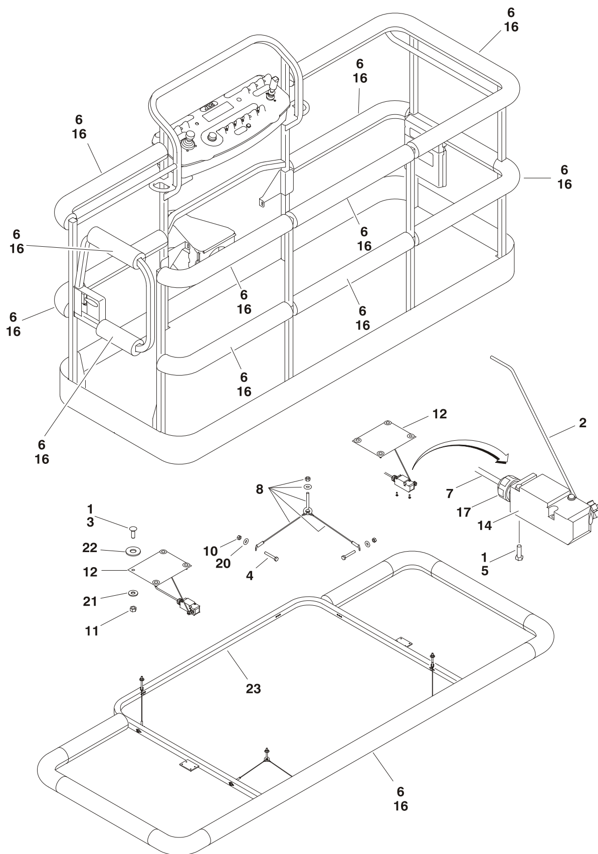
FIGURE 4-8. SOFT TOUCH SYSTEM INSTALLATION (OPTIONAL)
