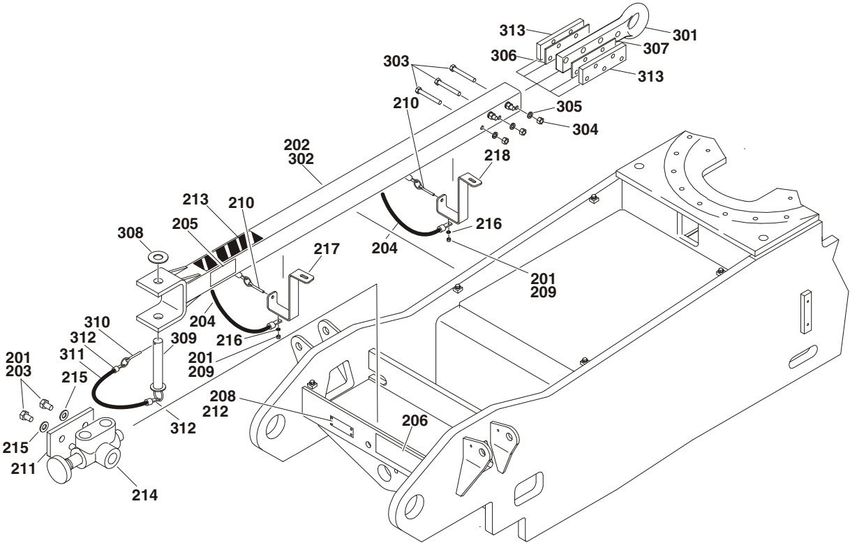
FIGURE 1-10. TOW PACKAGE INSTALLATION (2WS ONLY)
