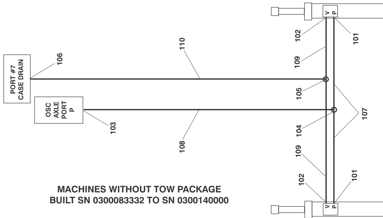
FIGURE 6-1. AXLE LOCKOUT HYDRAULIC DIAGRAM
