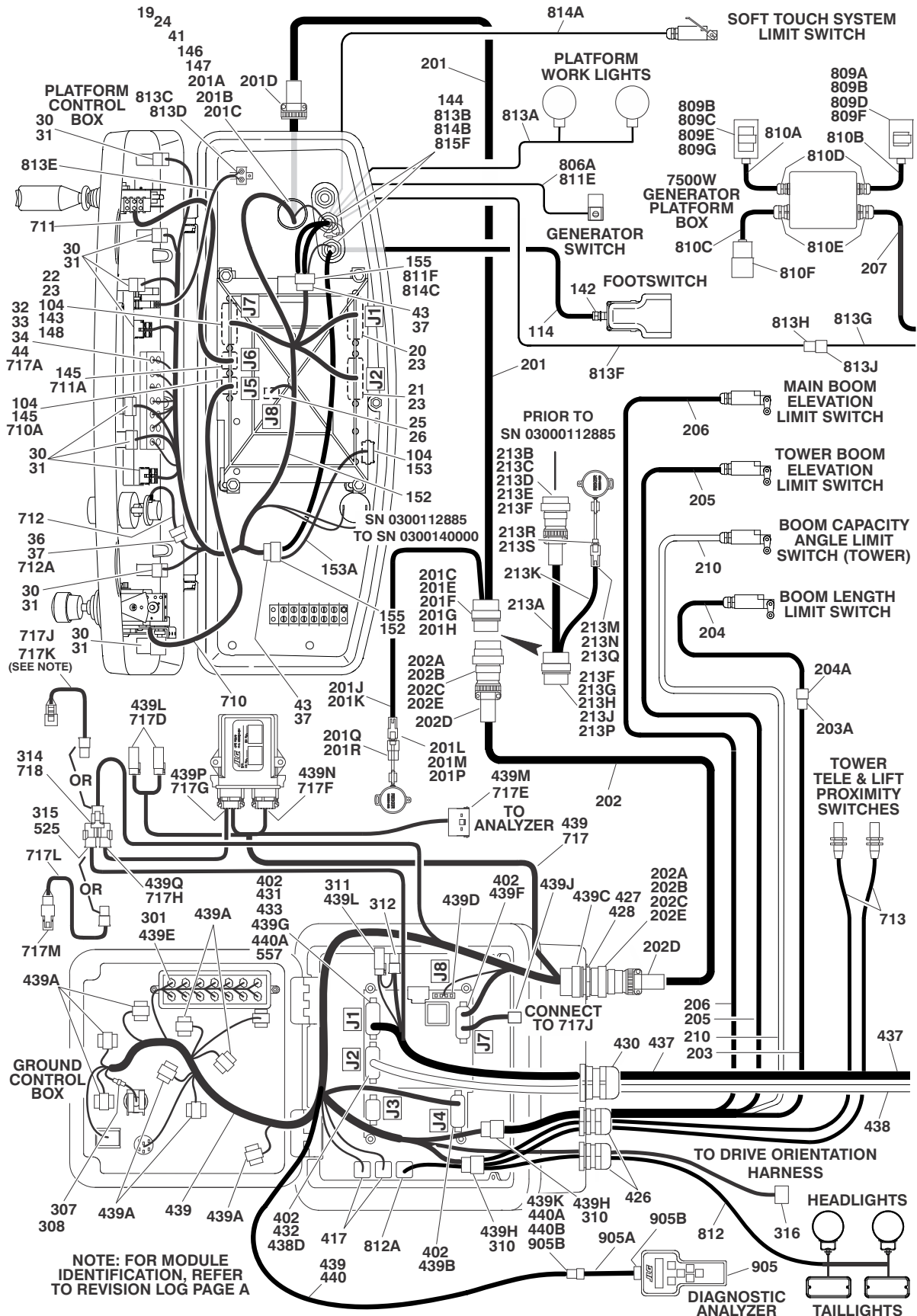
FIGURE 7-2. HARNESS COMPONENTS INSTALLATION WITHOUT UGM
