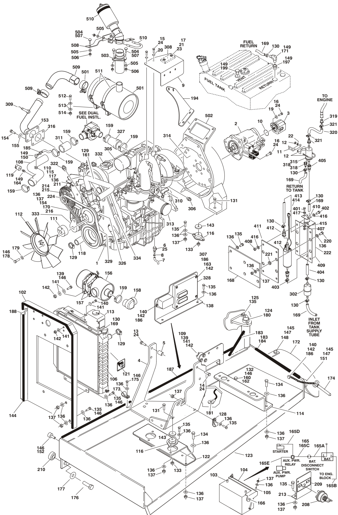
FIGURE 2-13. FORD ENGINE INSTALLATION - UL MACHINES (SN 0300069000 TO SN 0300077500)
