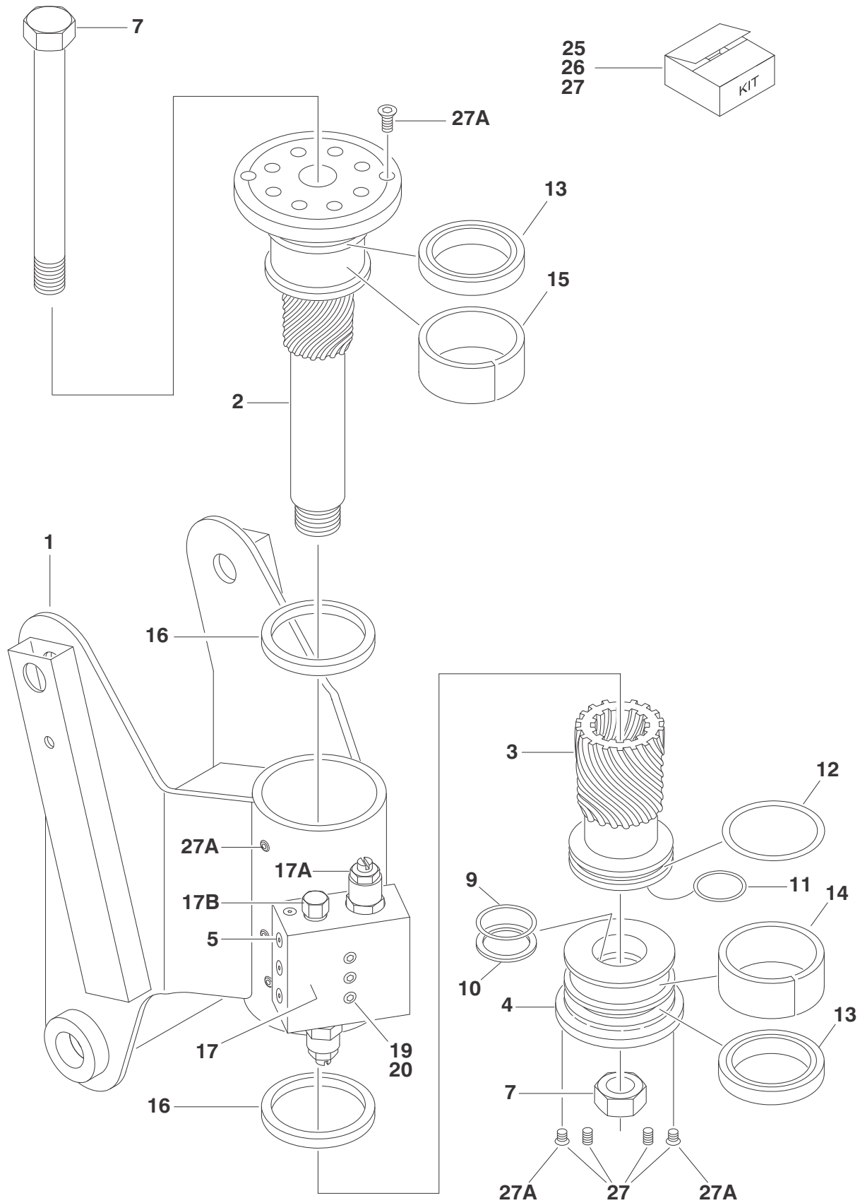
FIGURE 3-5. ROTATOR ASSEMBLY (FRONT ENTRY PLATFORM)
