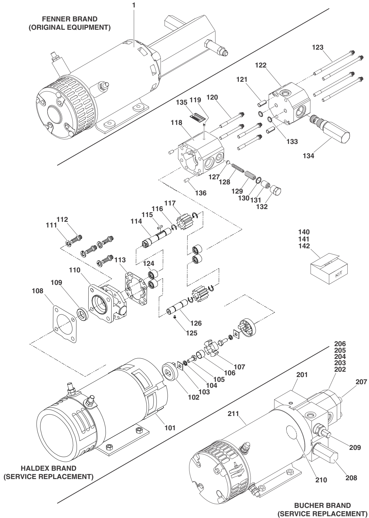
FIGURE 2-4. AUXILIARY PUMP ASSEMBLY (SN 03000109067 TO SN 0300140000)
