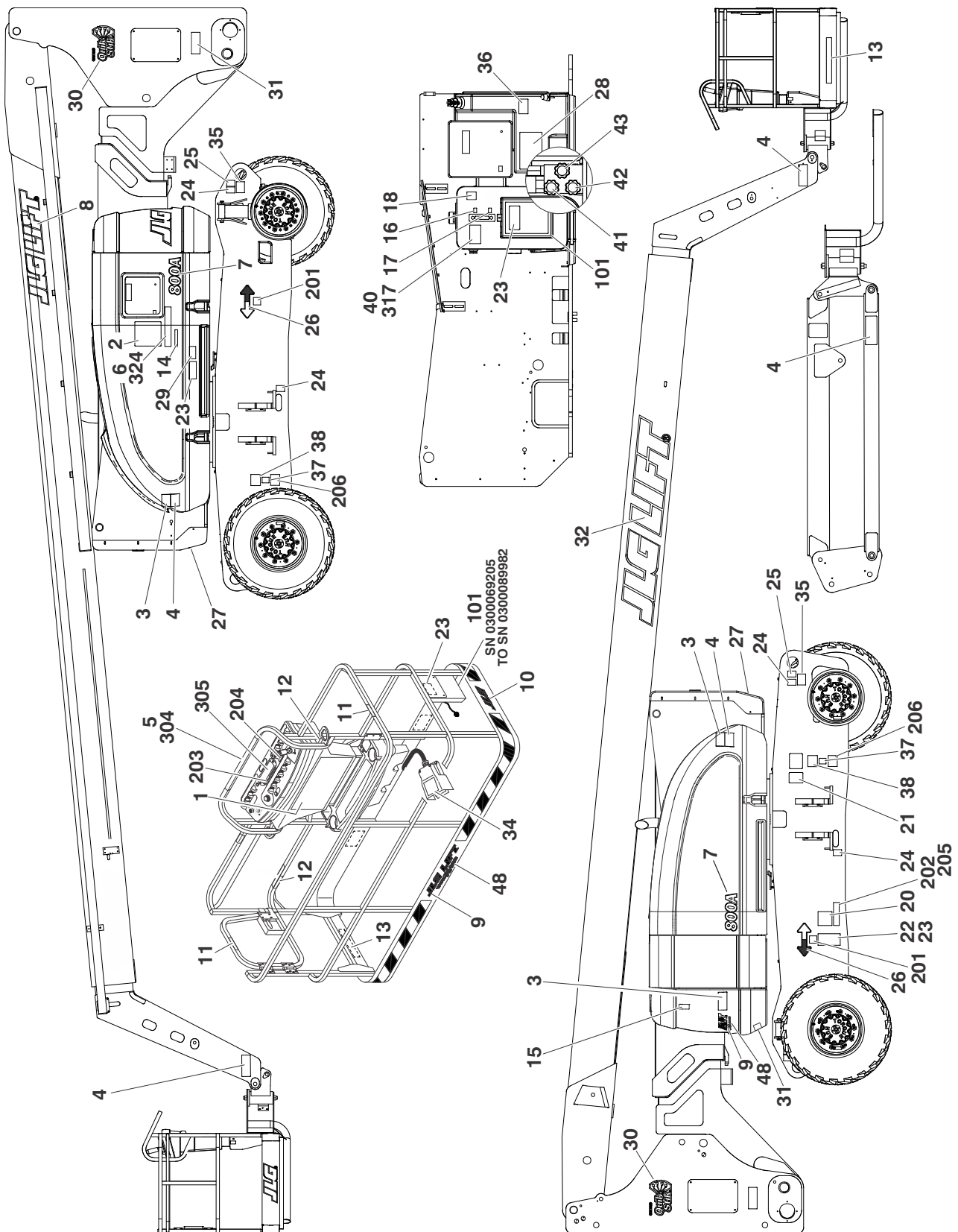
FIGURE 8-1. DECAL INSTALLATION (ANSI SPEC) (SN 0300069000 TO SN 0300089982)
