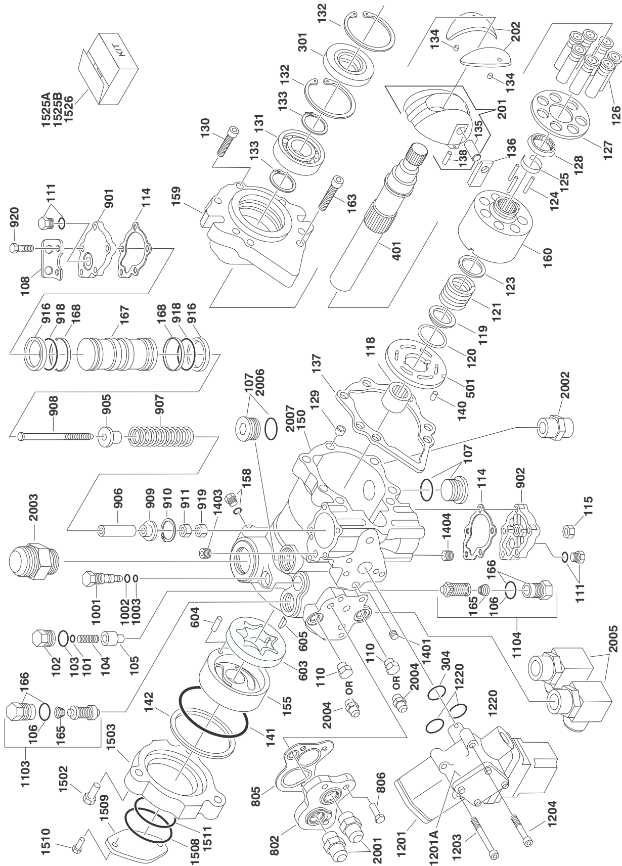
FIGURE 2-17. PISTON PUMP ASSEMBLY
