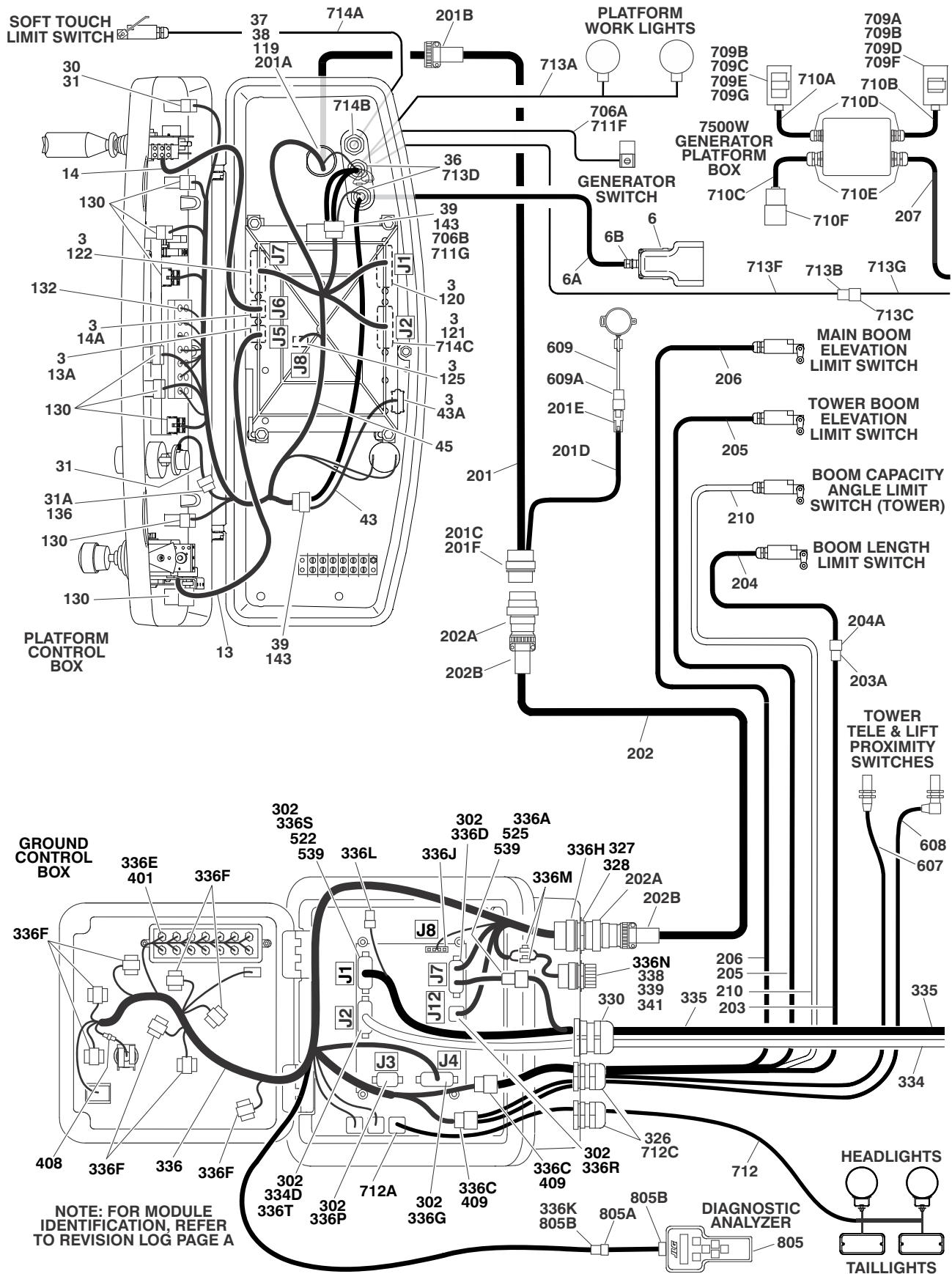
FIGURE 7-3. HARNESS COMPONENTS INSTALLATION WITH UGM
