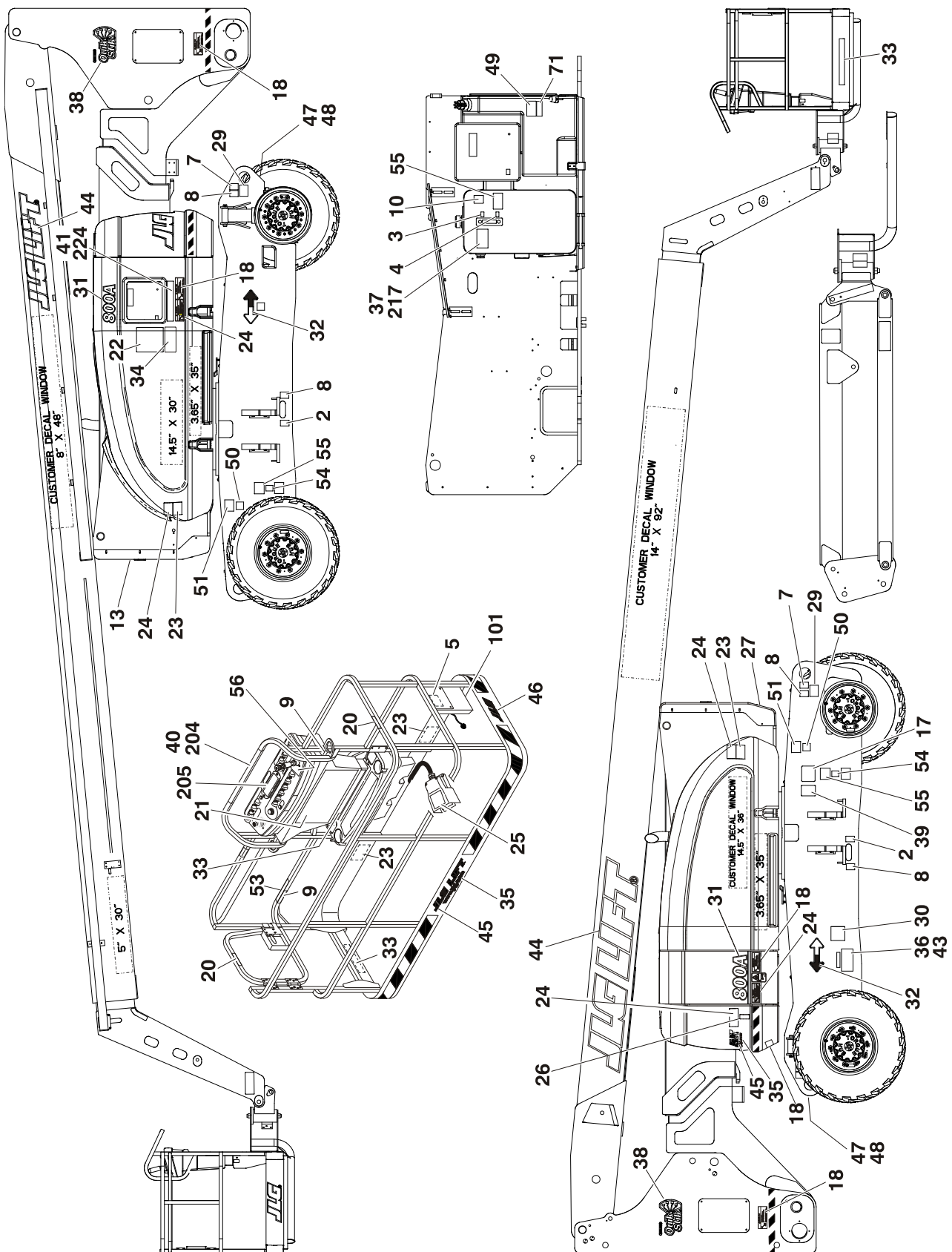
FIGURE 8-2. DECAL INSTALLATION (ANSI SPEC) (SN 0300089982 TO SN 0300140000)
