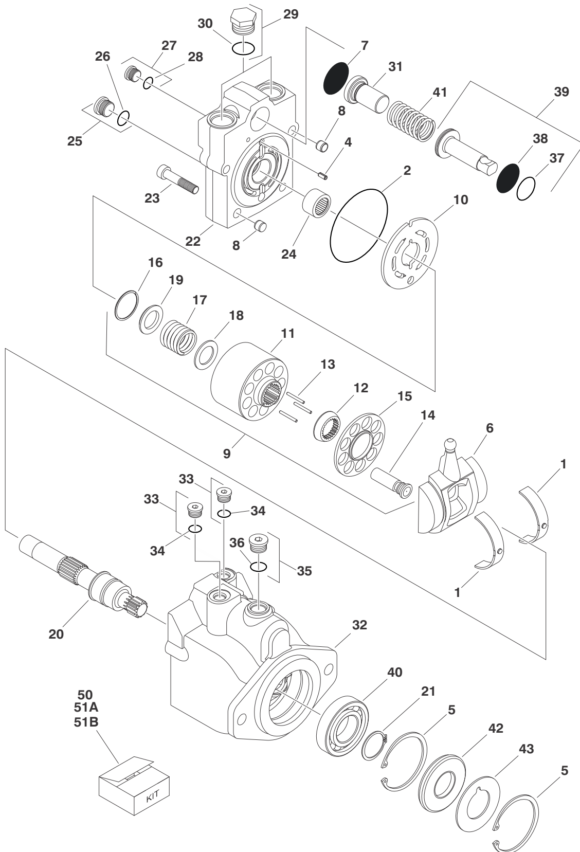
FIGURE 1-6. DRIVE MOTOR ASSEMBLY (ORIGINAL EQUIPMENT) (SN 0300083332 TO SN 0300140000) (4 BOLT ASSEMBLY)
