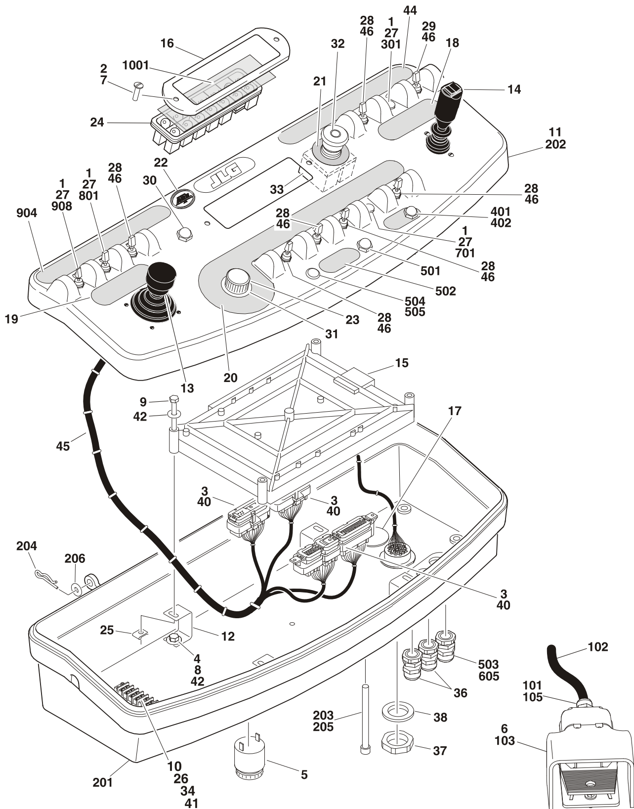
FIGURE 4-5. PLATFORM CONSOLE ASSEMBLY (SN 0300137975 TO SN 0300140000)
