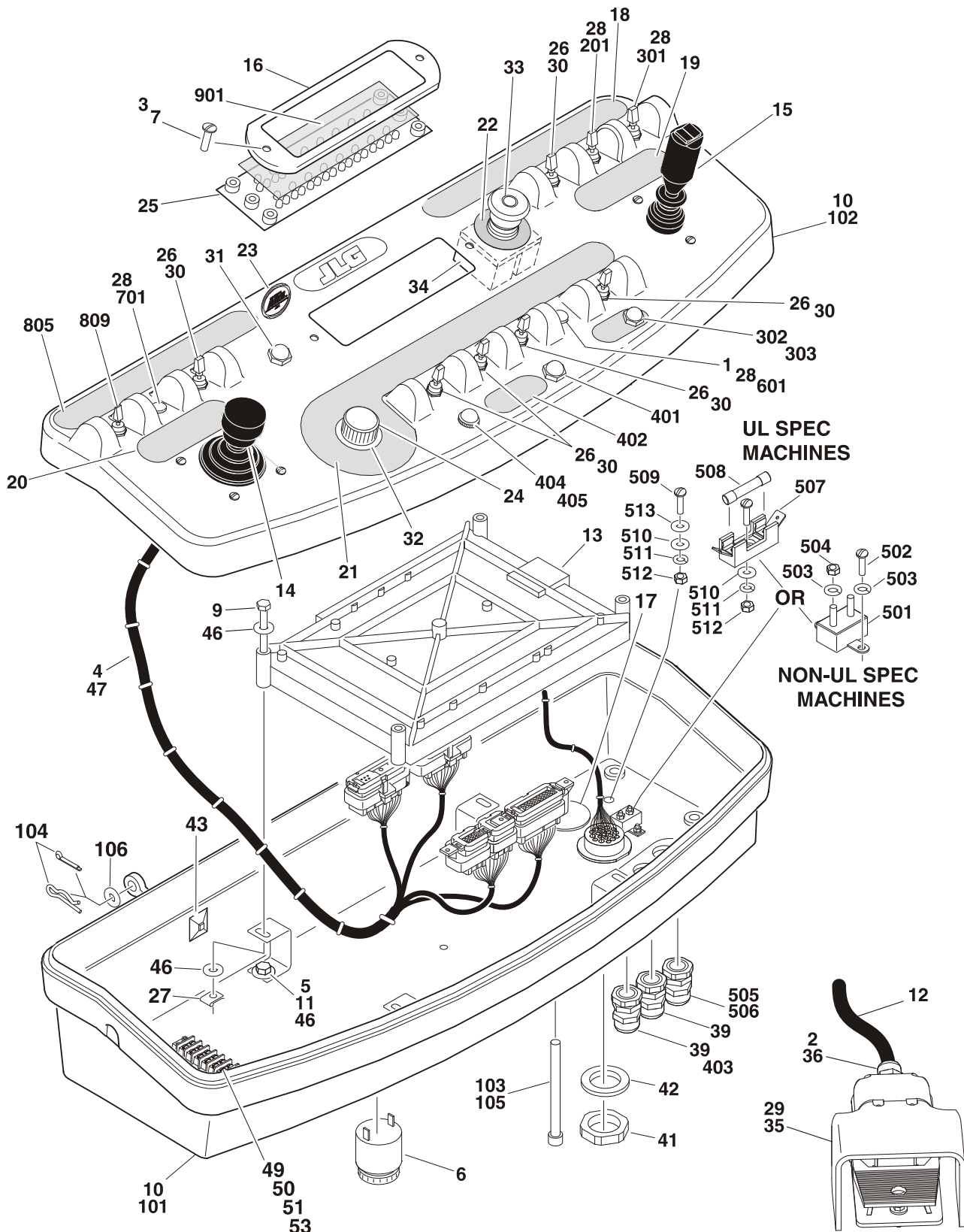
FIGURE 4-4. PLATFORM CONSOLE ASSEMBLY (SN 0300069000 TO SN 0300137975)
