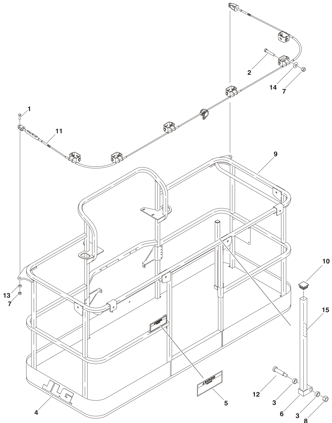
FIGURE 4-3. PLATFORM COMPONENTS INSTALLATION (FALL ARREST FOR PLATFORM)
