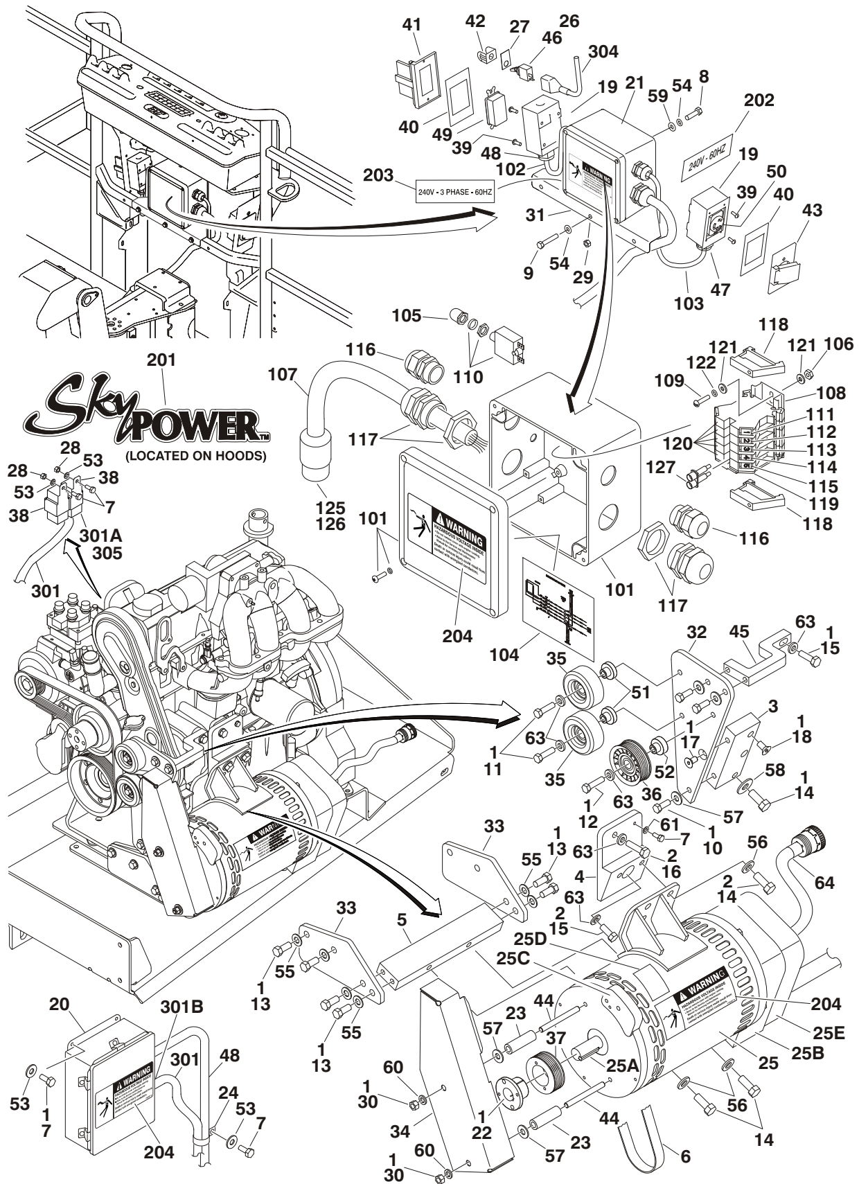
FIGURE 2-34. 7500W SKYPOWER GENERATOR INSTALLATION - FORD MACHINES (ANSI & CSA SPECS)
