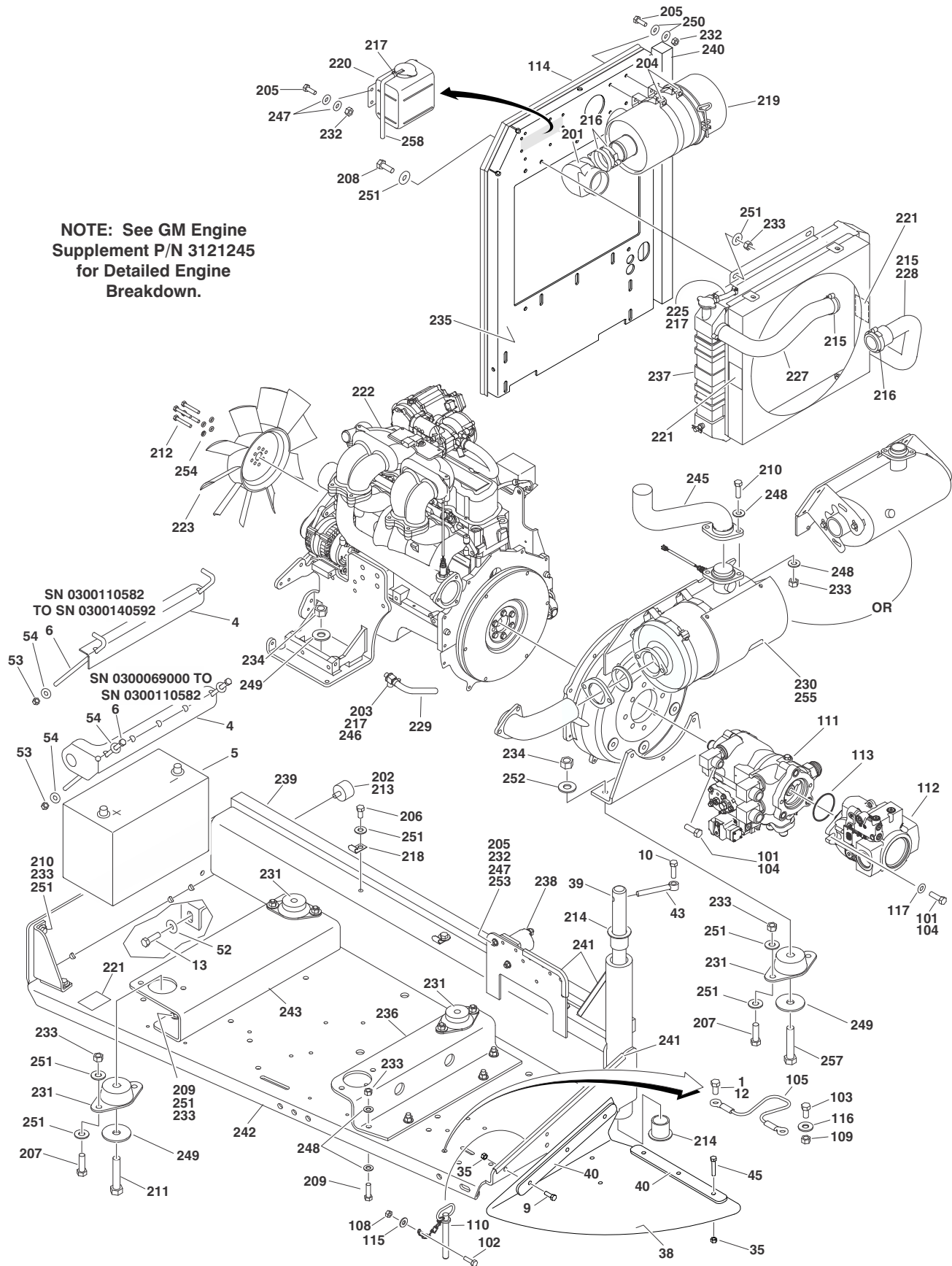
FIGURE 2-16. GM ENGINE INSTALLATION (SN 0300069000 TO SN 0300140000)
