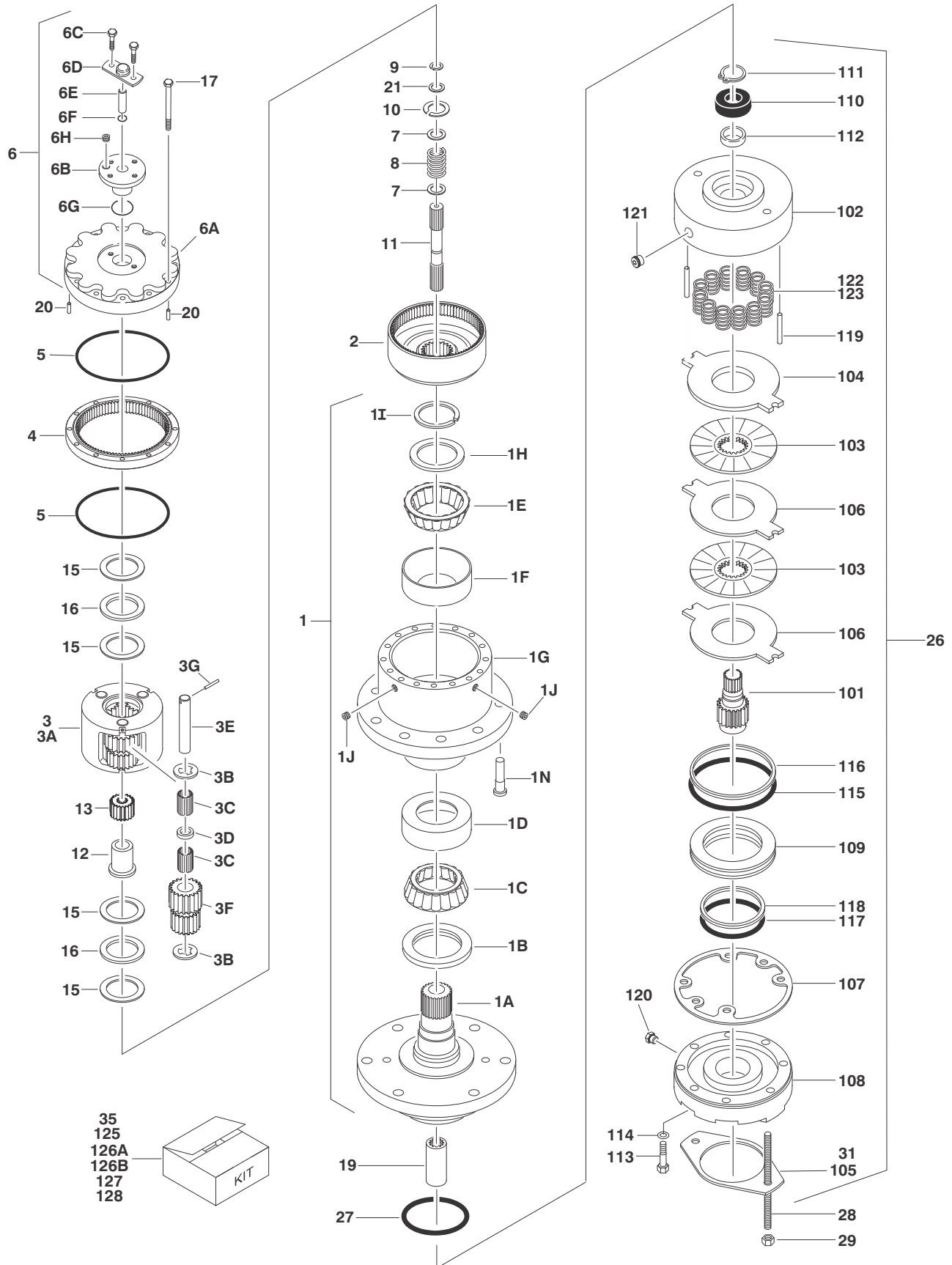
FIGURE 1-4. DRIVE HUB ASSEMBLY (SN 0300083332 TO SN 0300140000)
