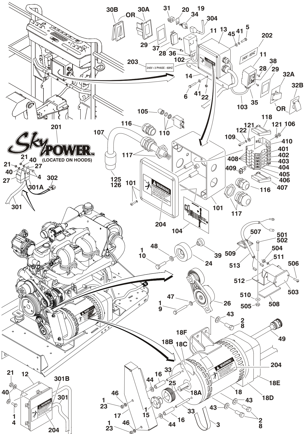
FIGURE 2-35. 7500W SKYPOWER GENERATOR INSTALLATION - GM MACHINES (ANSI & CSA SPECS)
