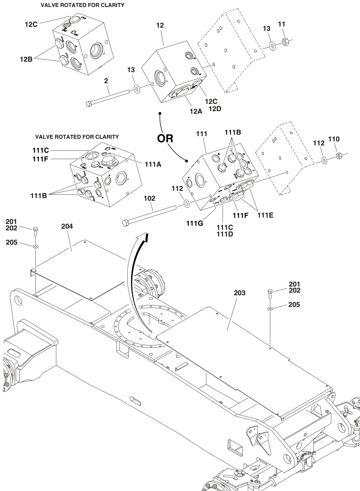
FIGURE 1-9. DRIVE VALVES & SHIELDS INSTALLATIONS (SN 0300083332 TO SN 0300140000)
