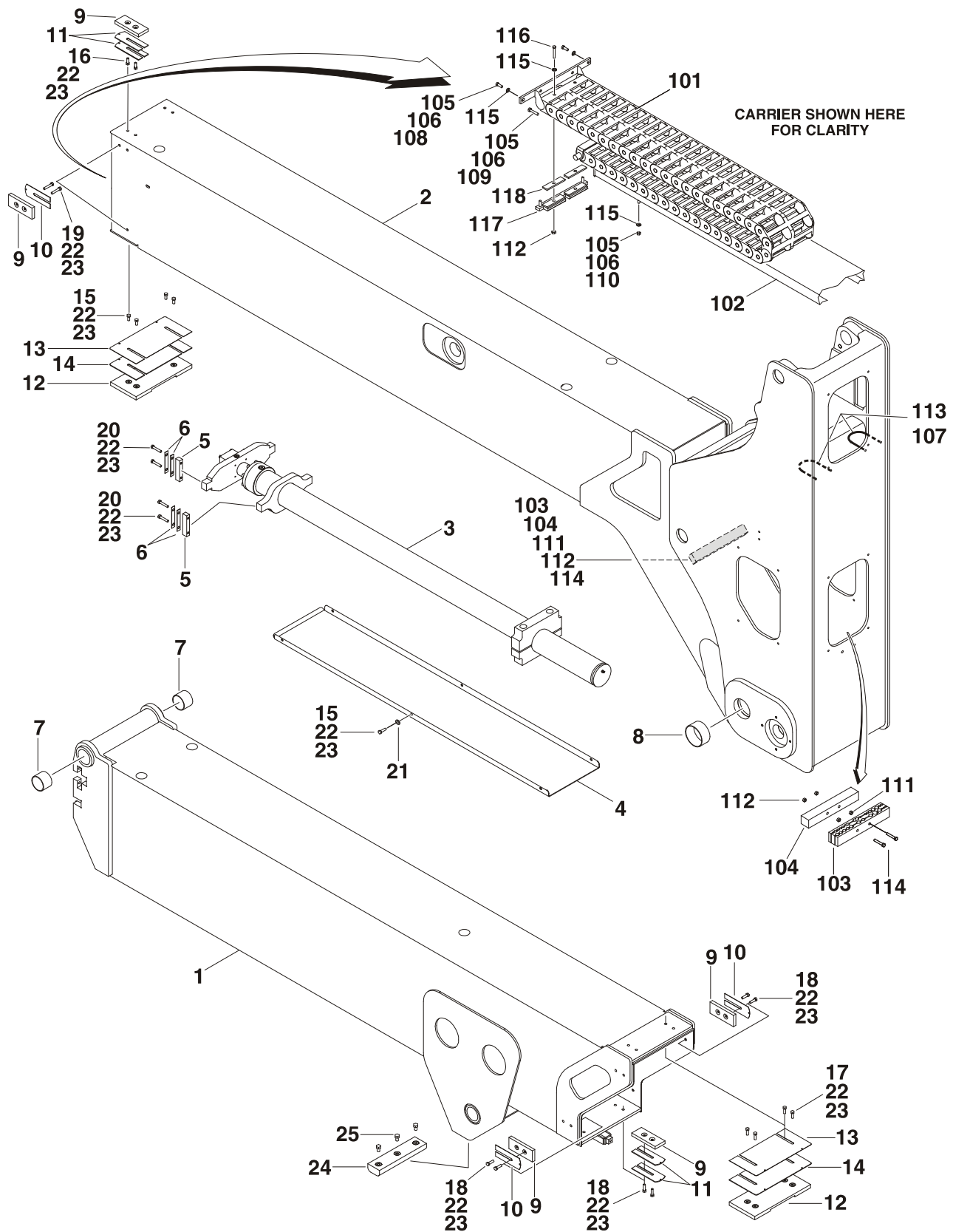
FIGURE 3-3. TOWER BOOM ASSEMBLY
