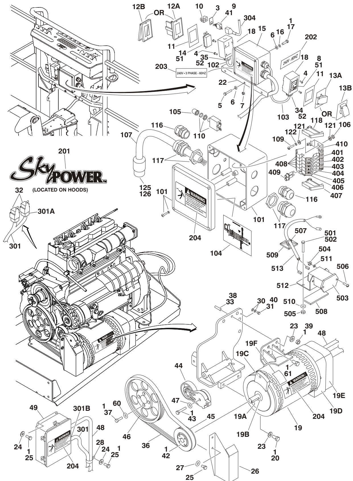
FIGURE 2-33. 7500W SKYPOWER GENERATOR INSTALLATION - CATERPILLAR AND DEUTZ MACHINES (ANSI & CSA SPECS)
