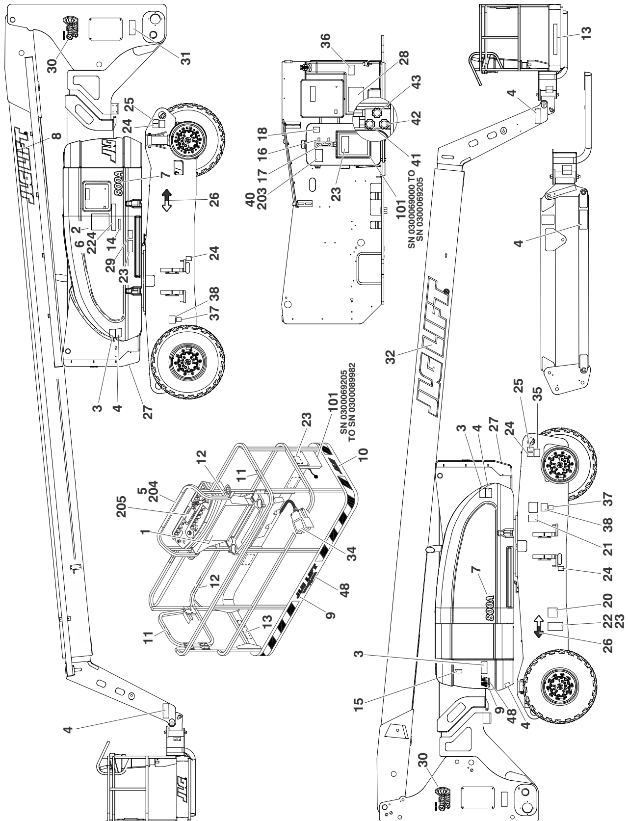
FIGURE 8-3. DECAL INSTALLATION (COUNTRY SPEC) (SN 0300069000 TO SN 0300089982)
