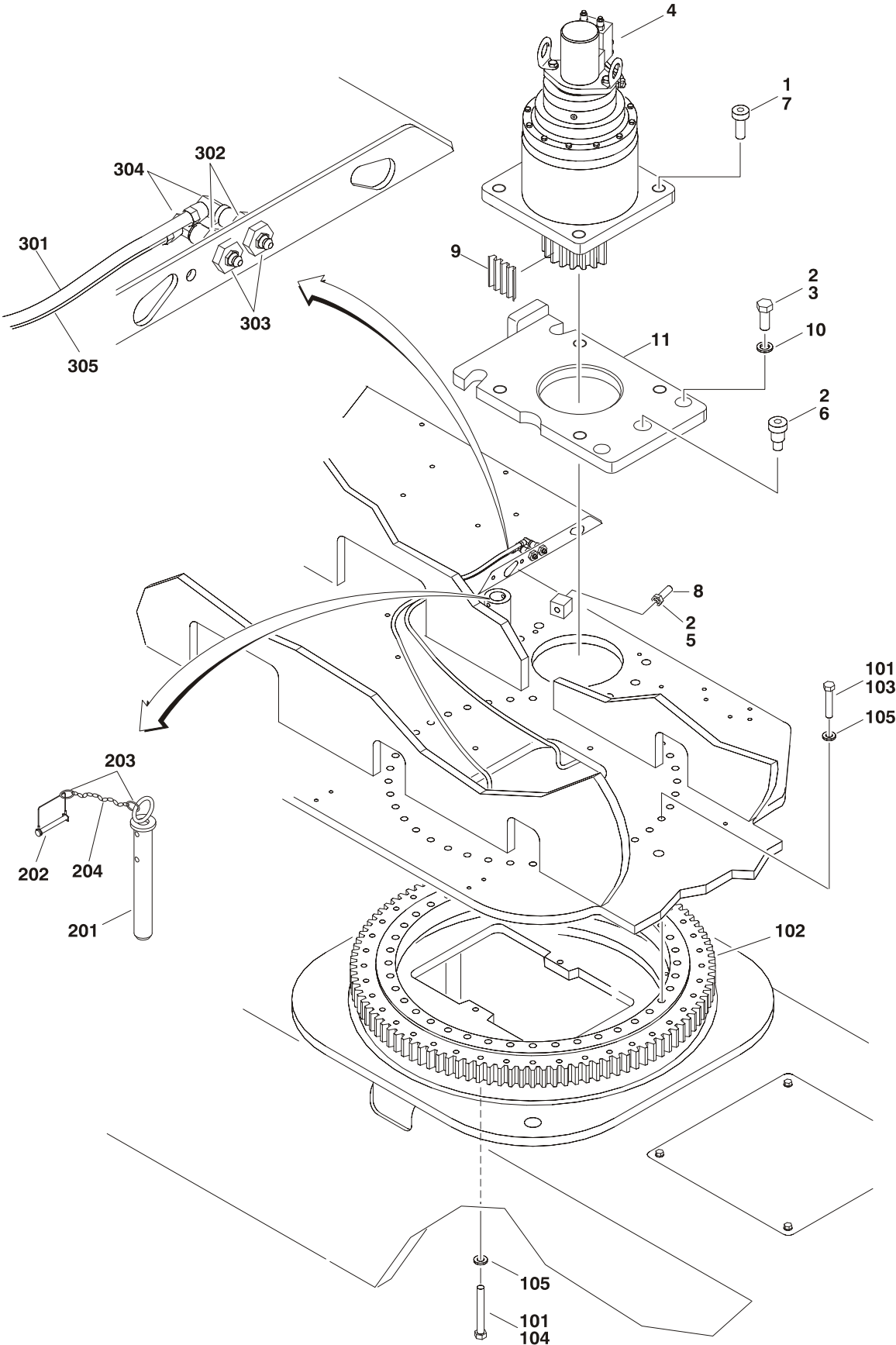
FIGURE 2-5. TURNTABLE BEARING AND SWING DRIVE INSTALLATION
