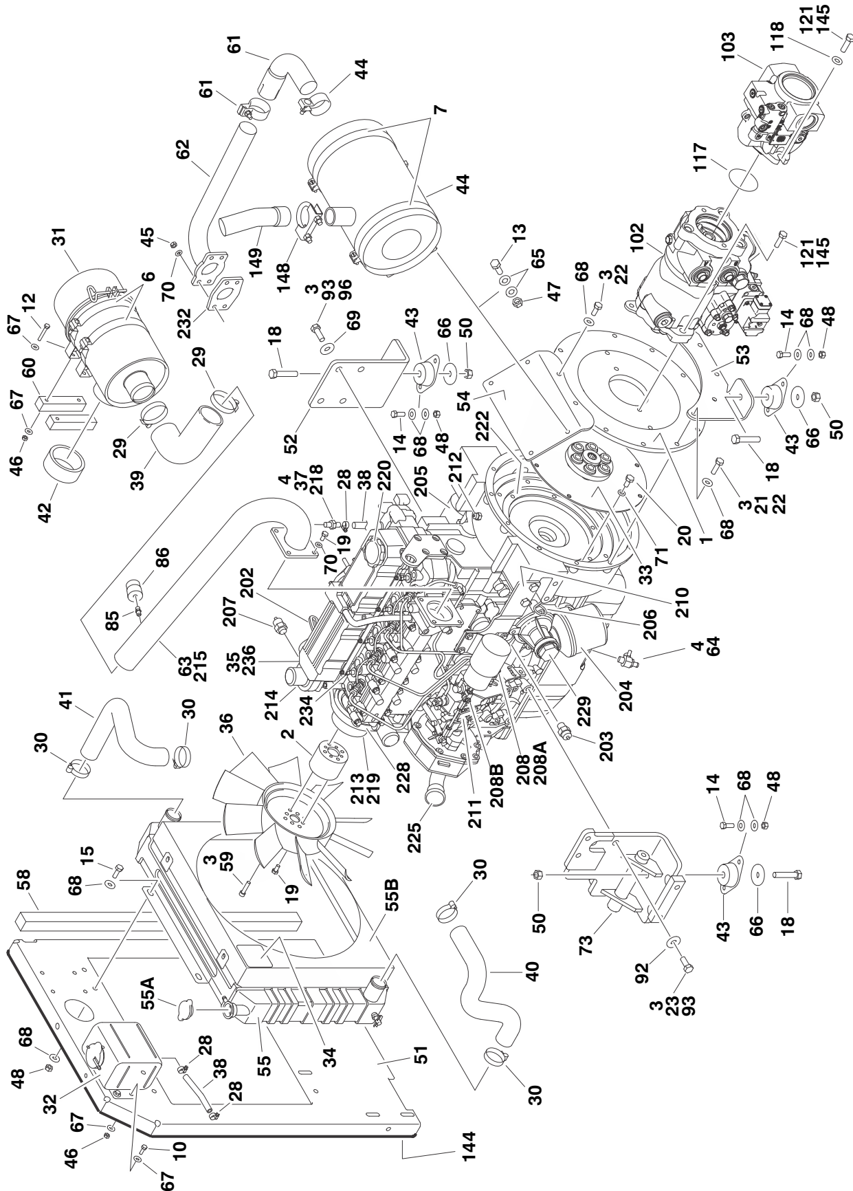
FIGURE 2-8. CATERPILLAR ENGINE INSTALLATION (SN 0300069000 TO SN 0300139400)
