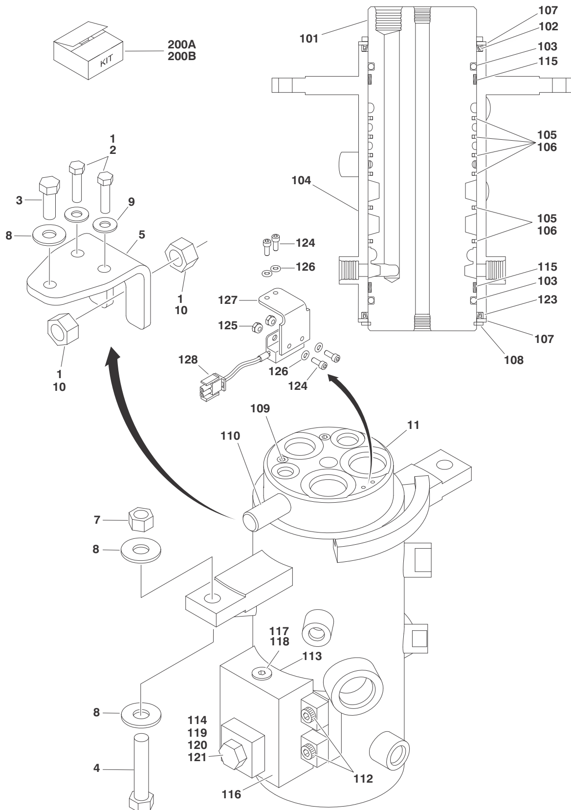
FIGURE 2-21. ROTARY COUPLING INSTALLATION (SN 0300137975 TO SN 0300140000)
