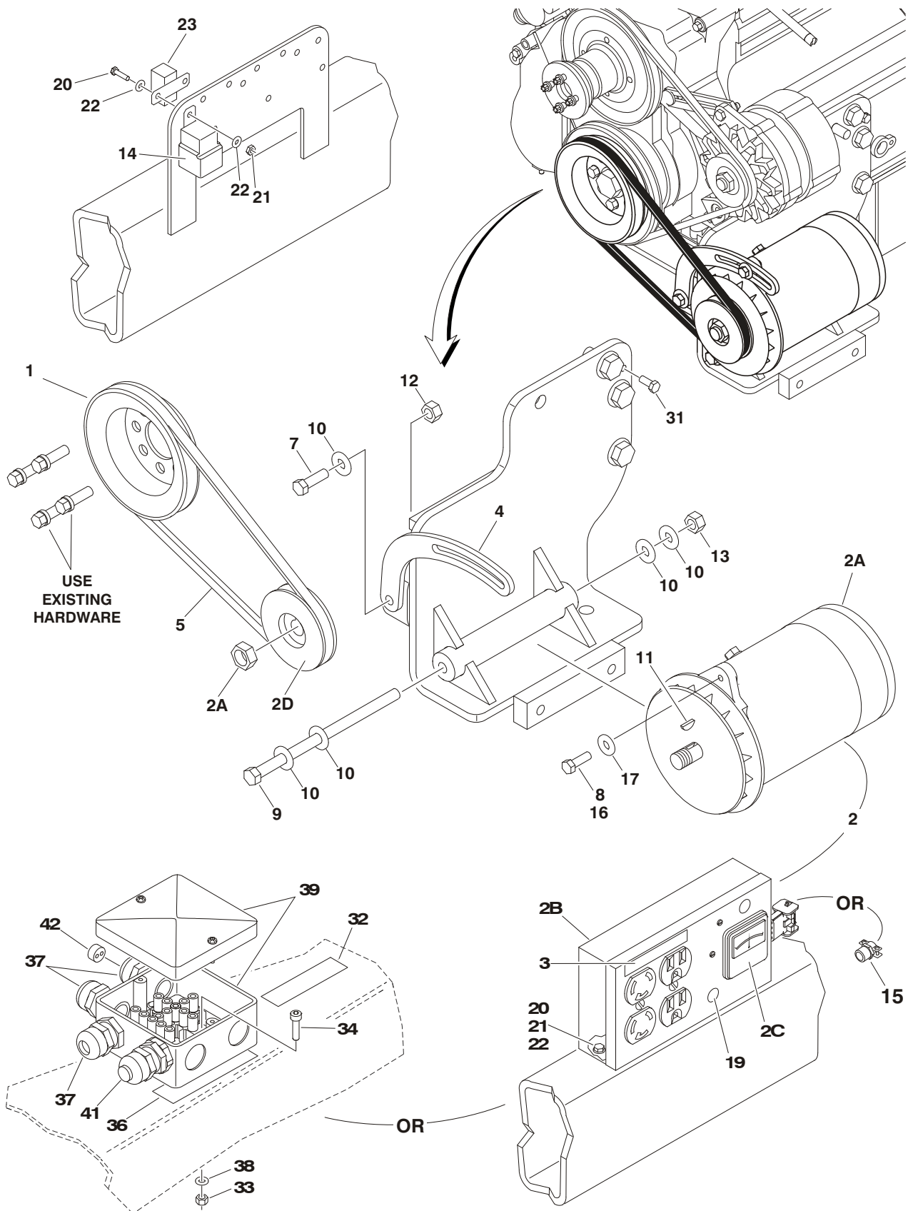
FIGURE 2-29. 2500W GENERATOR INSTALLATION - DEUTZ MACHINES (OPTIONAL)
