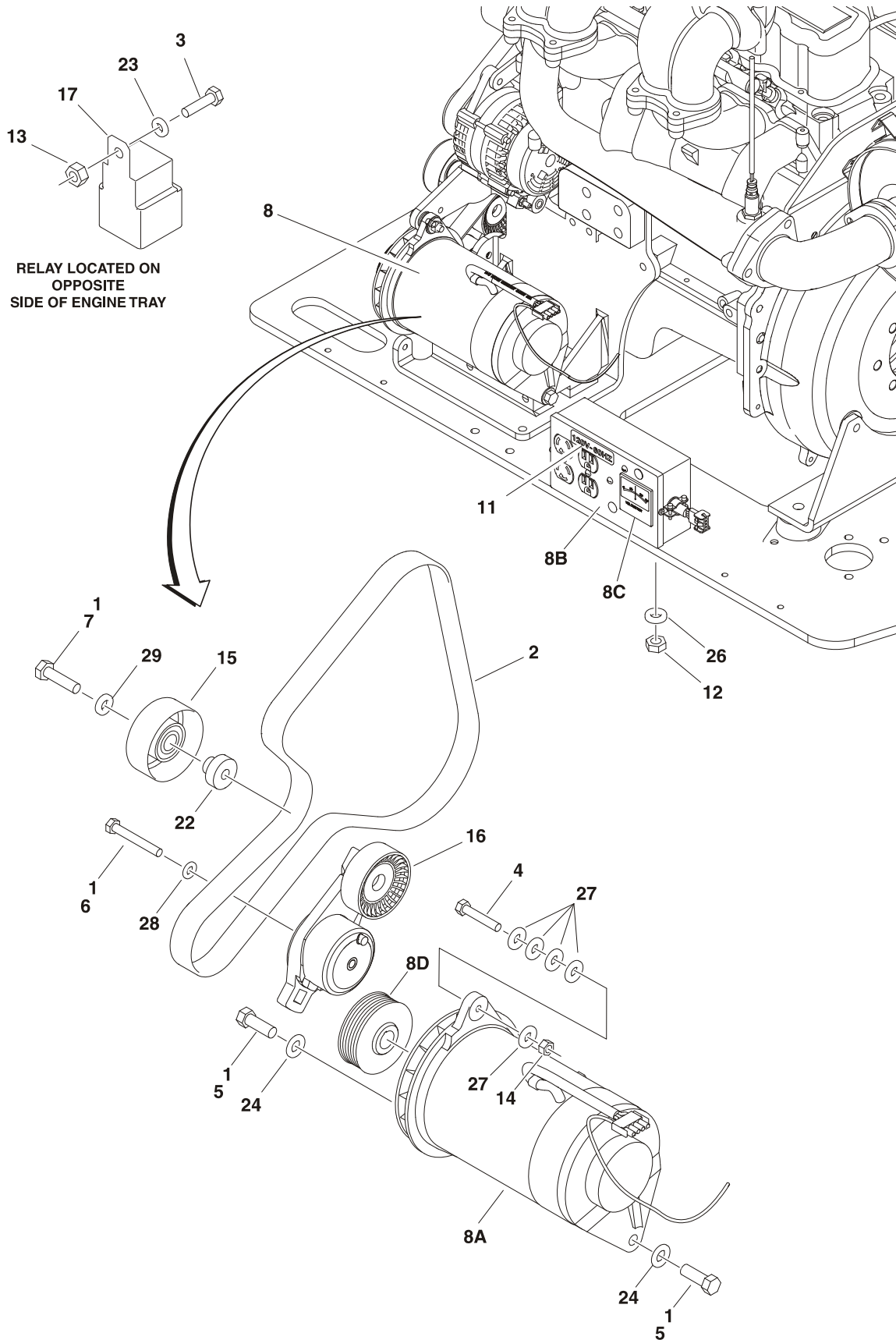
FIGURE 2-32. 2500W GENERATOR INSTALLATION - GM MACHINES (OPTIONAL)
