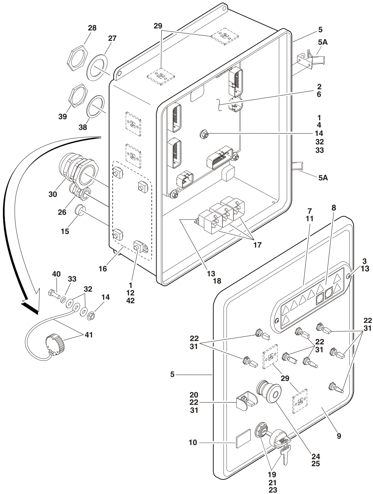
FIGURE 2-23. GROUND CONTROL BOX ASSEMBLY (WITH UGM)
