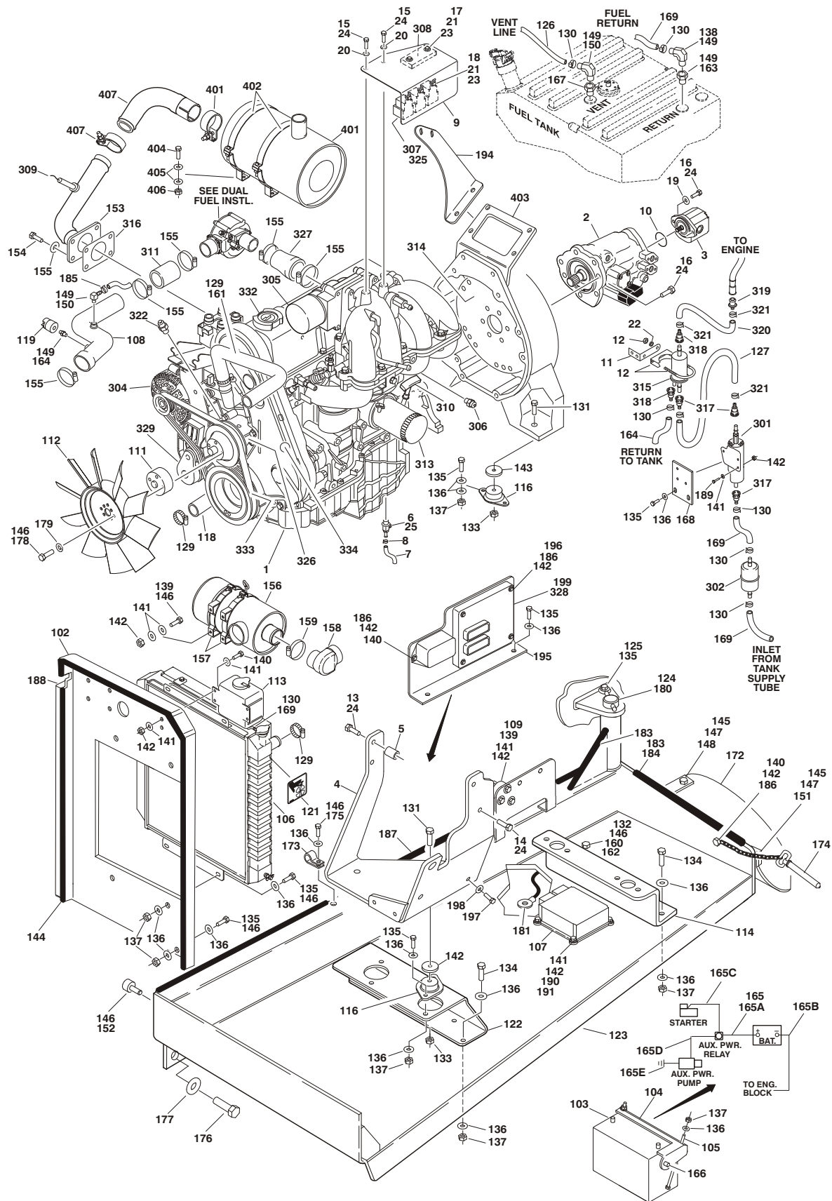
FIGURE 2-12. FORD ENGINE INSTALLATION - NON-UL SPEC MACHINES (SN 0300069000 TO SN 0300077500)
