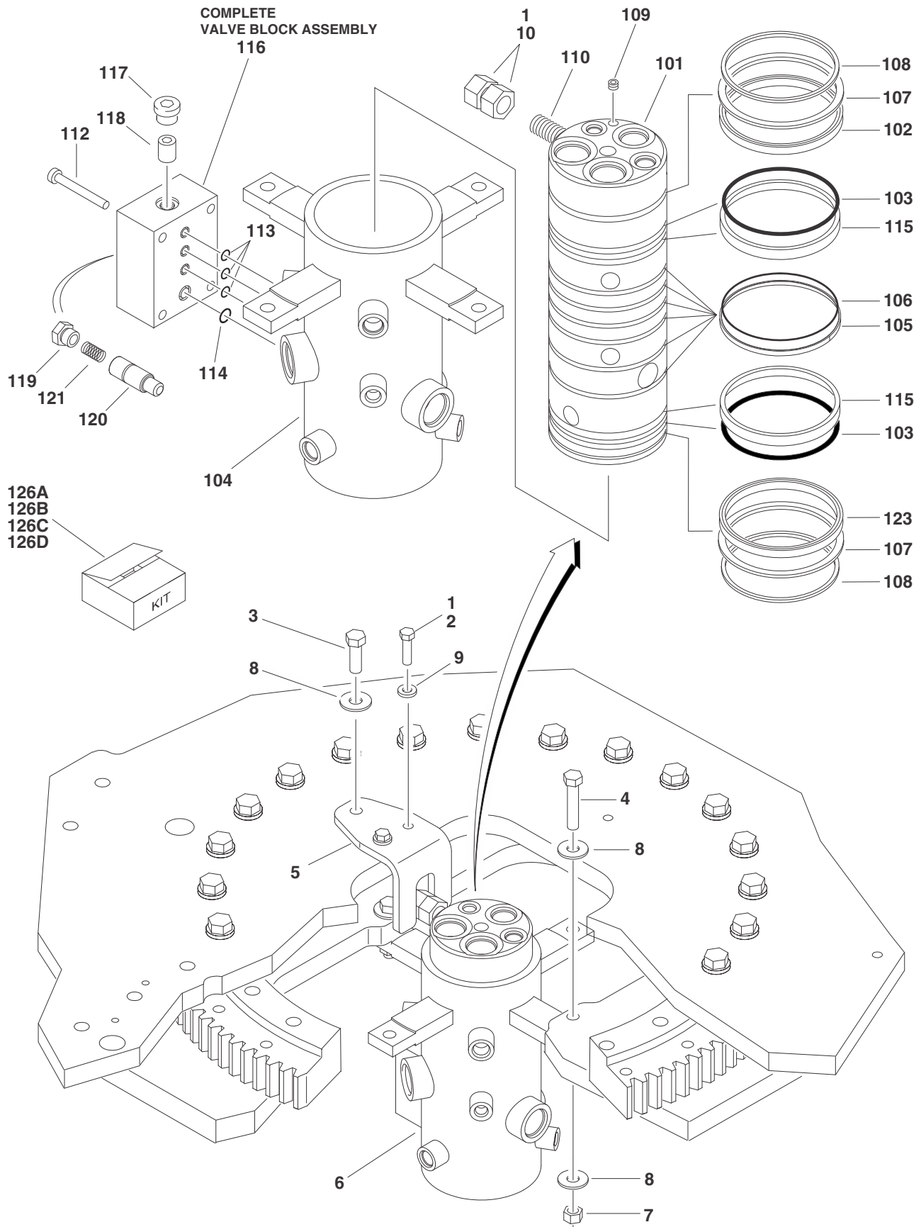
FIGURE 2-20. ROTARY COUPLING INSTALLATION (SN 0300083332 TO SN 0300137975)
