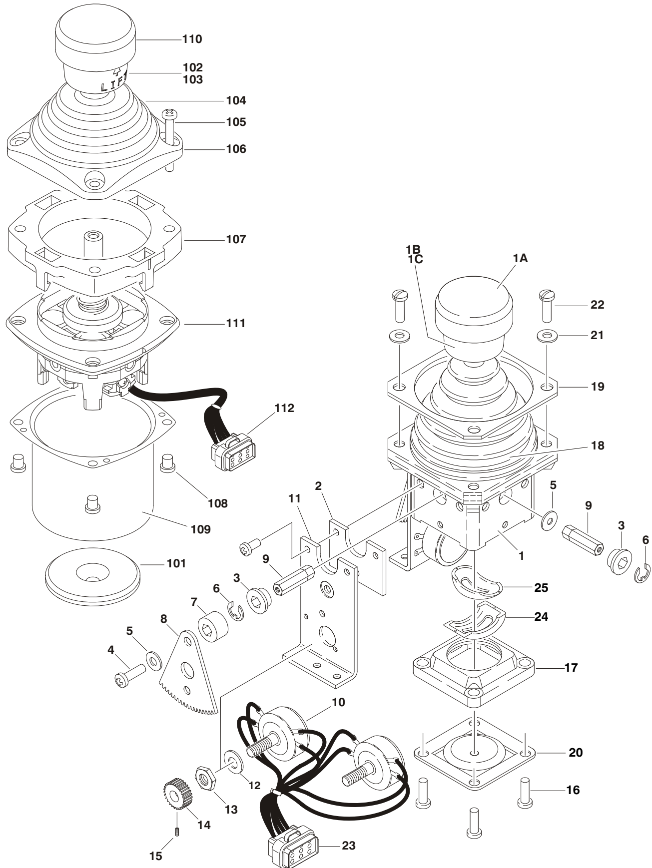
FIGURE 4-6. CONTROLLER ASSEMBLY (SWING & LIFT)
