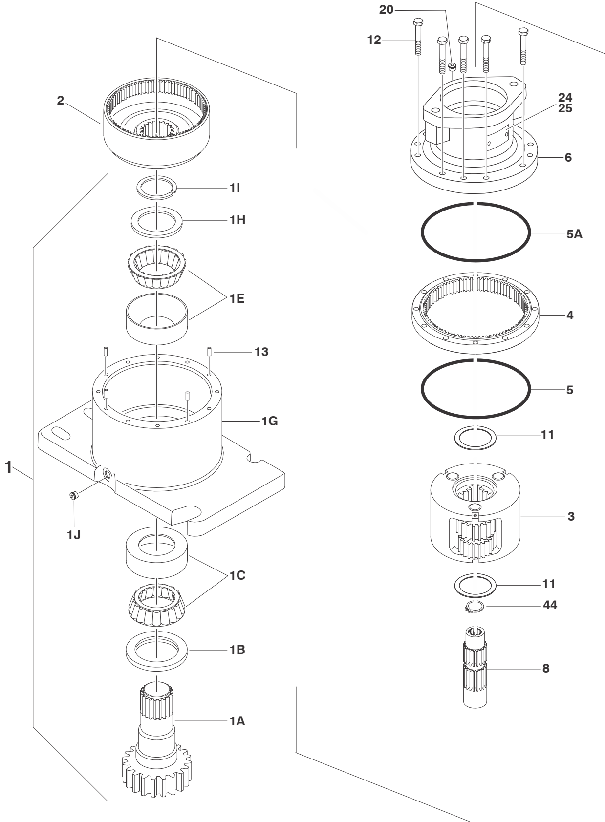
FIGURE 2-7. SWING MOTOR/HUB ASSEMBLY (SN 0300134353 TO SN 0300140000)
