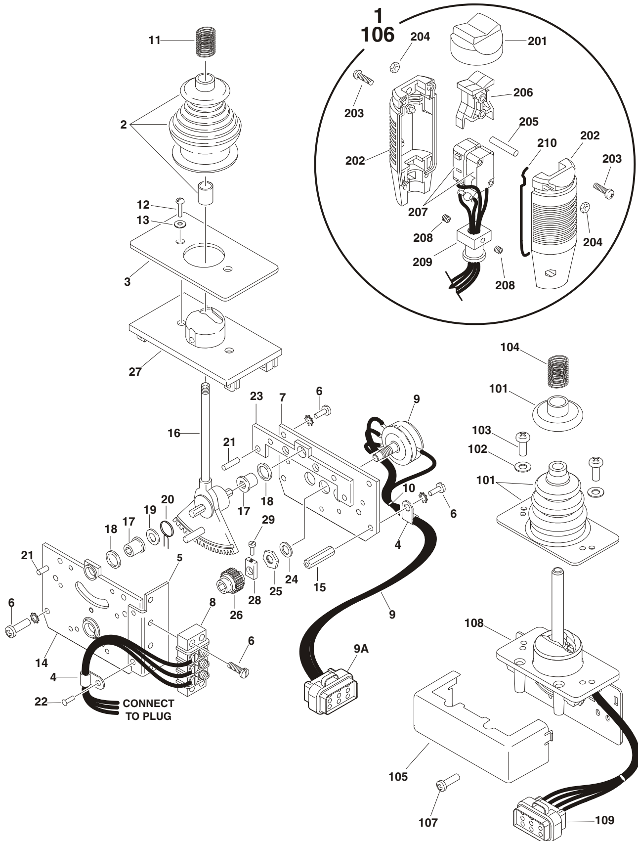
FIGURE 4-7. CONTROLLER ASSEMBLY (DRIVE & STEER)
