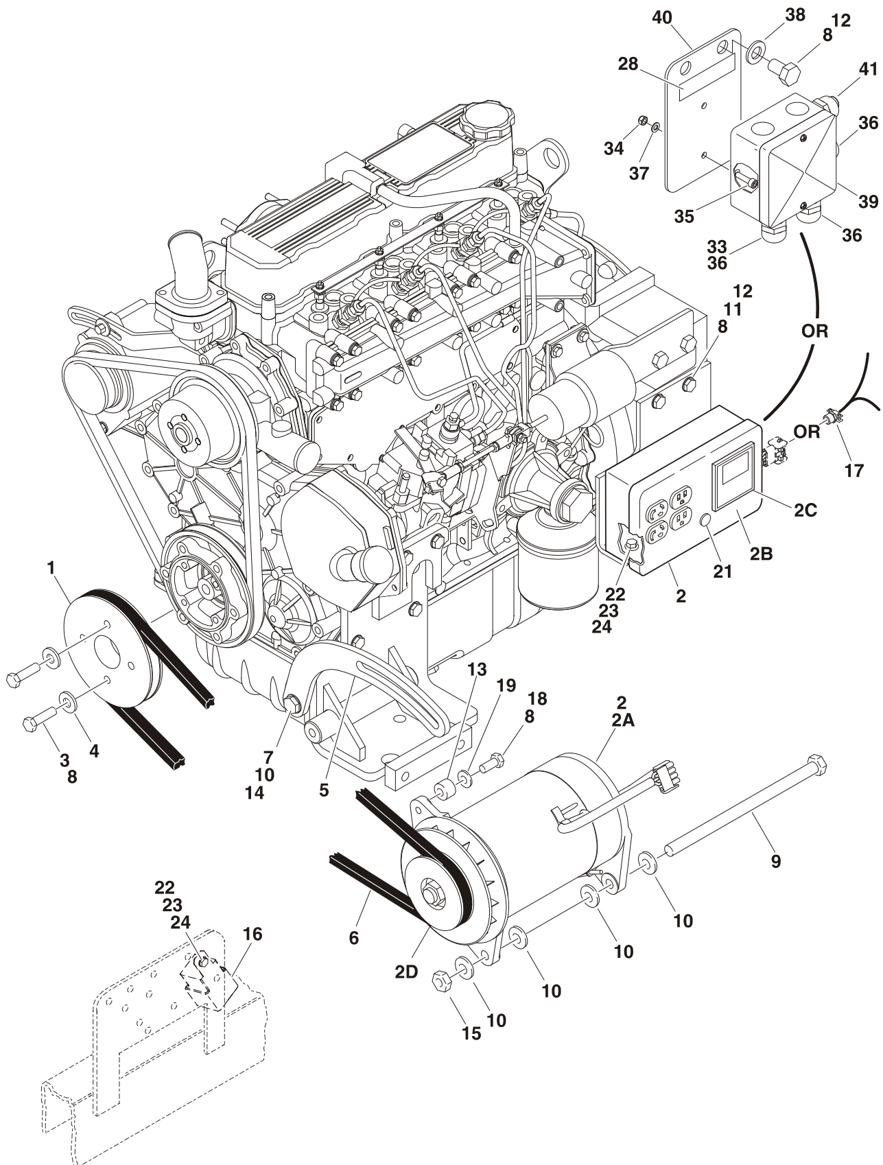
FIGURE 2-28. 2500W GENERATOR INSTALLATION - CATERPILLAR MACHINES (OPTIONAL)
