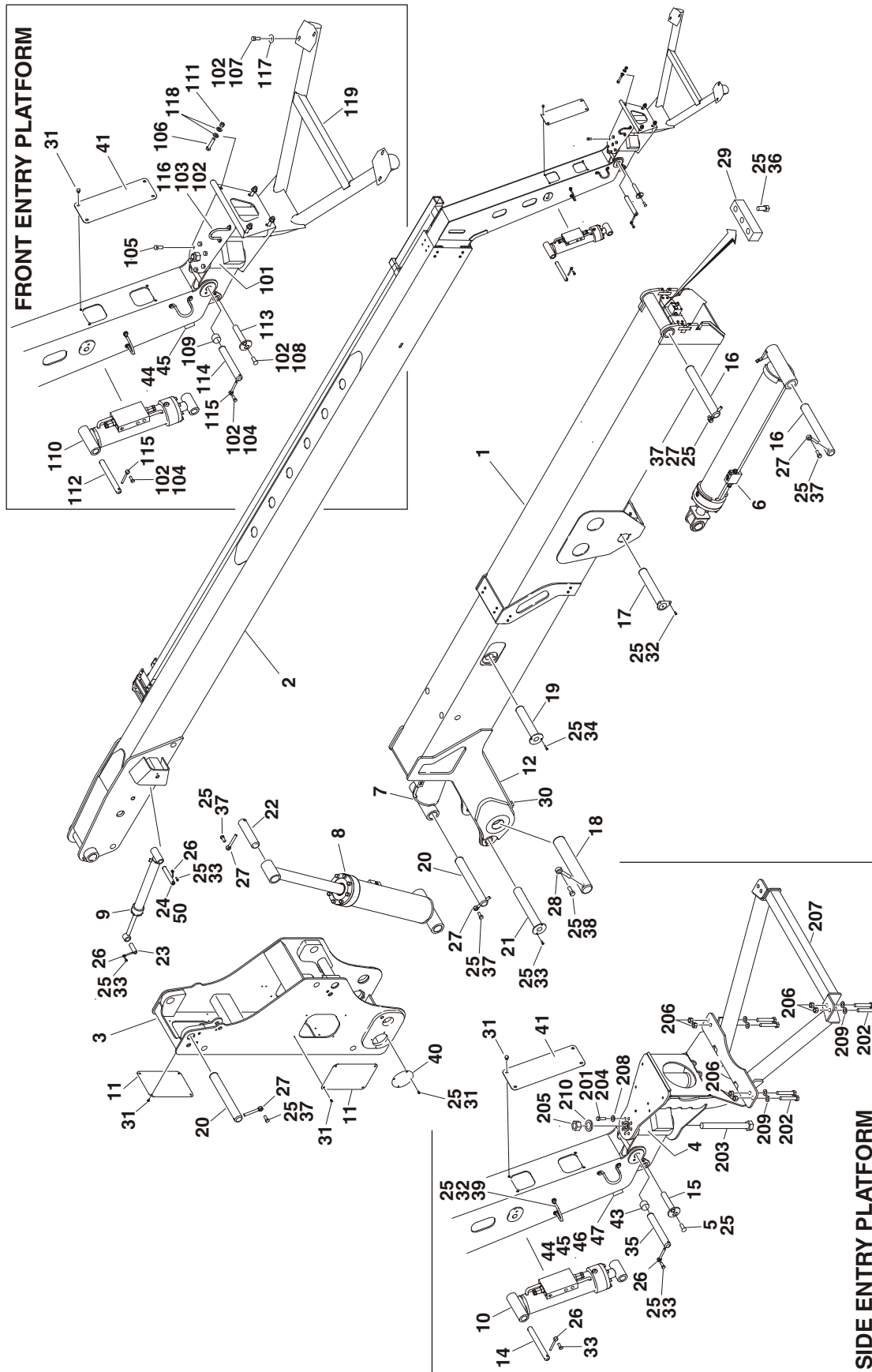
FIGURE 3-1. BOOM AND CYLINDER INSTALLATION - 800A
