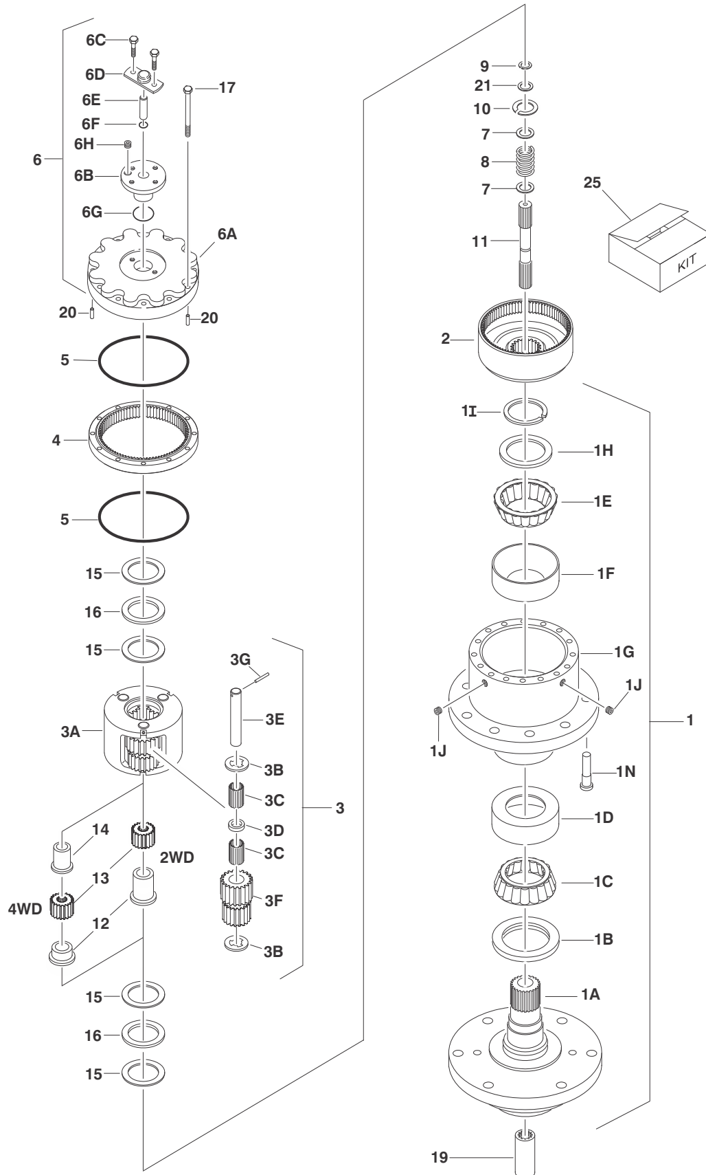
FIGURE 1-3. DRIVE HUB ASSEMBLIES (SN 0300069000 TO SN 0300083332)
